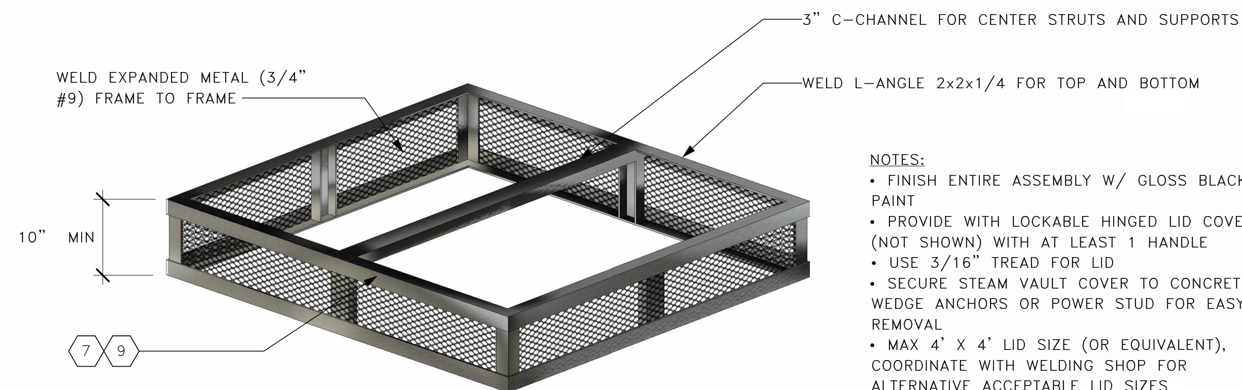
4 STEAM VAULT COVER WITH VENTED OPENING - ISOMETRIC
