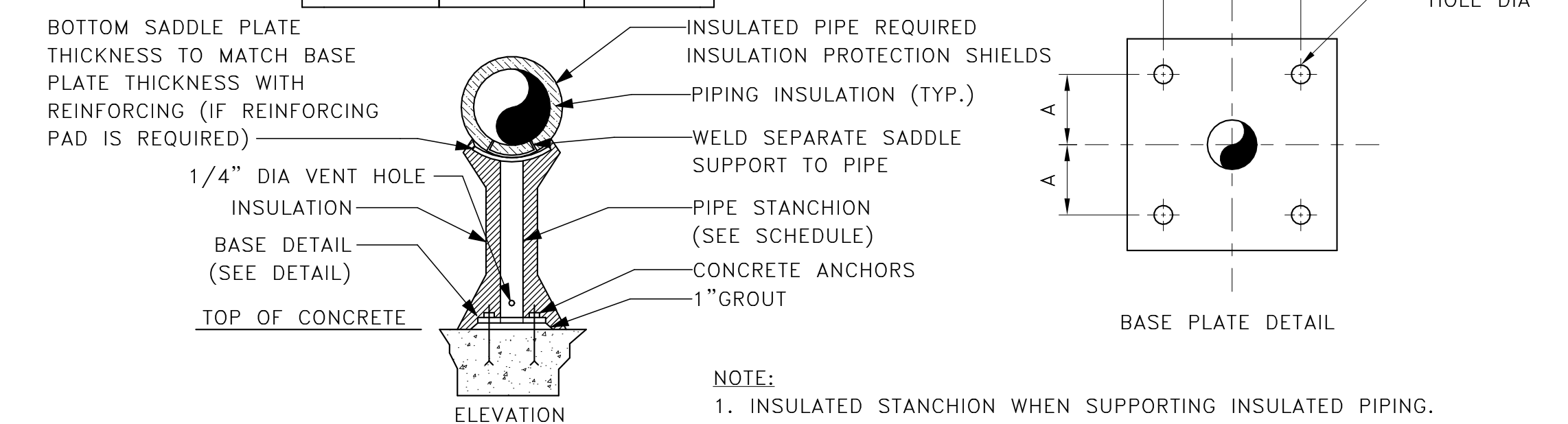
5 PIPE STANCHION ANCHOR SADDLE SUPPORT M-1.1 SCALE: NONE
