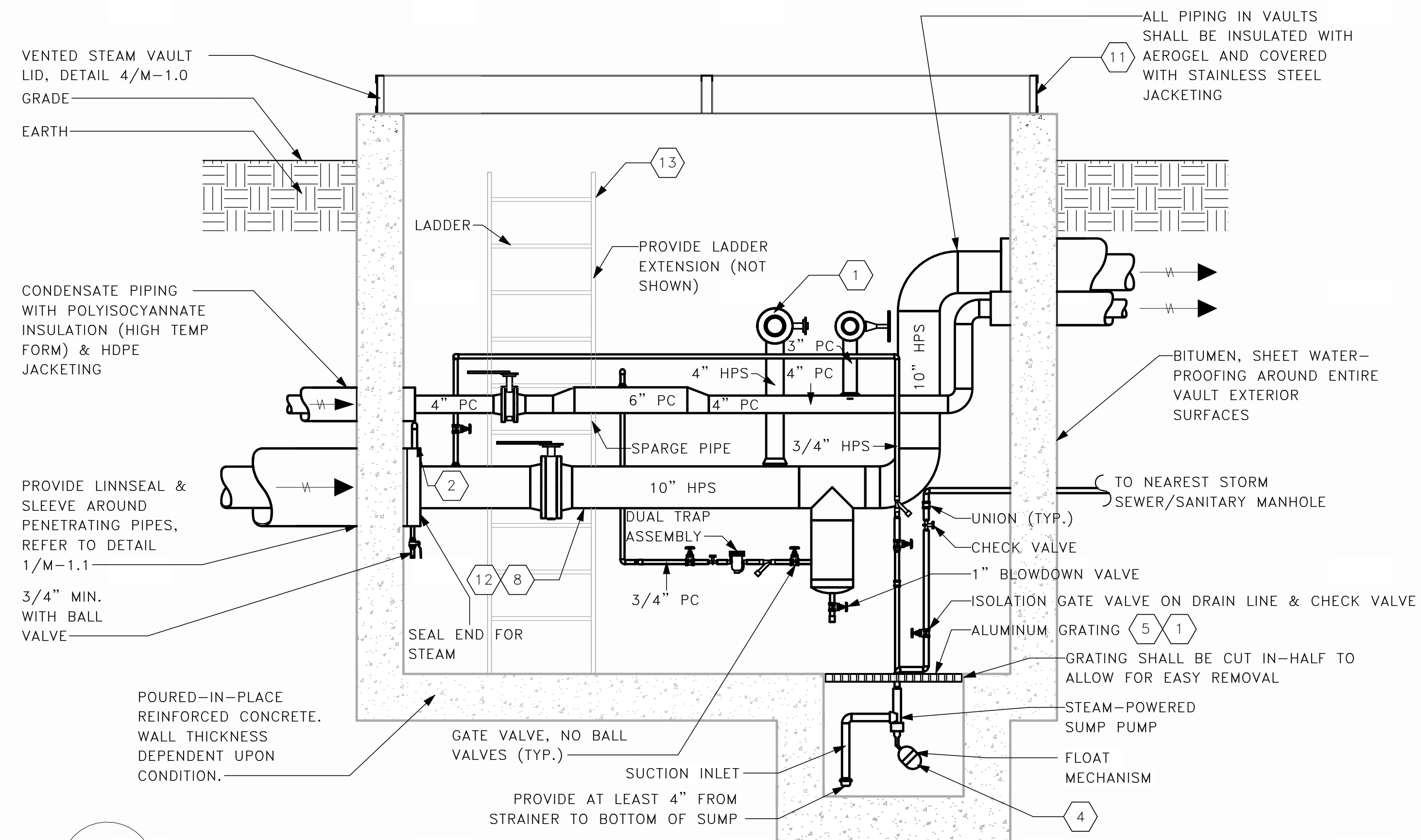
2 EXAMPLE STEAM VAULT SECTION VIEW (WITH VENTED COVER)
