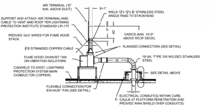
TYPICAL DETAIL - FUME HOOD EXHAUST FAN SUPPORT FRAME SCALE: NONE
